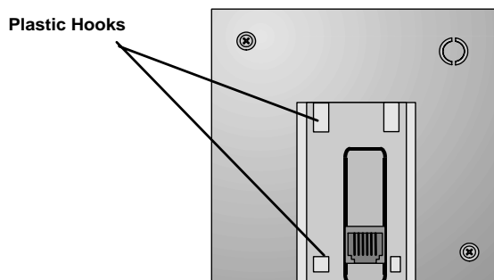
Figure 17 Plastic Hooks on Rear of KIRK Repeater
